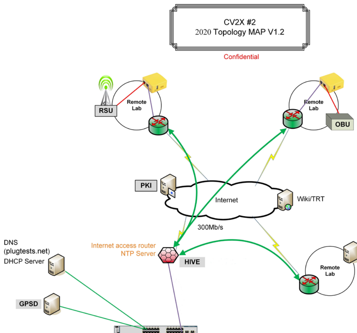
Figure 2. Test Infrastructure
