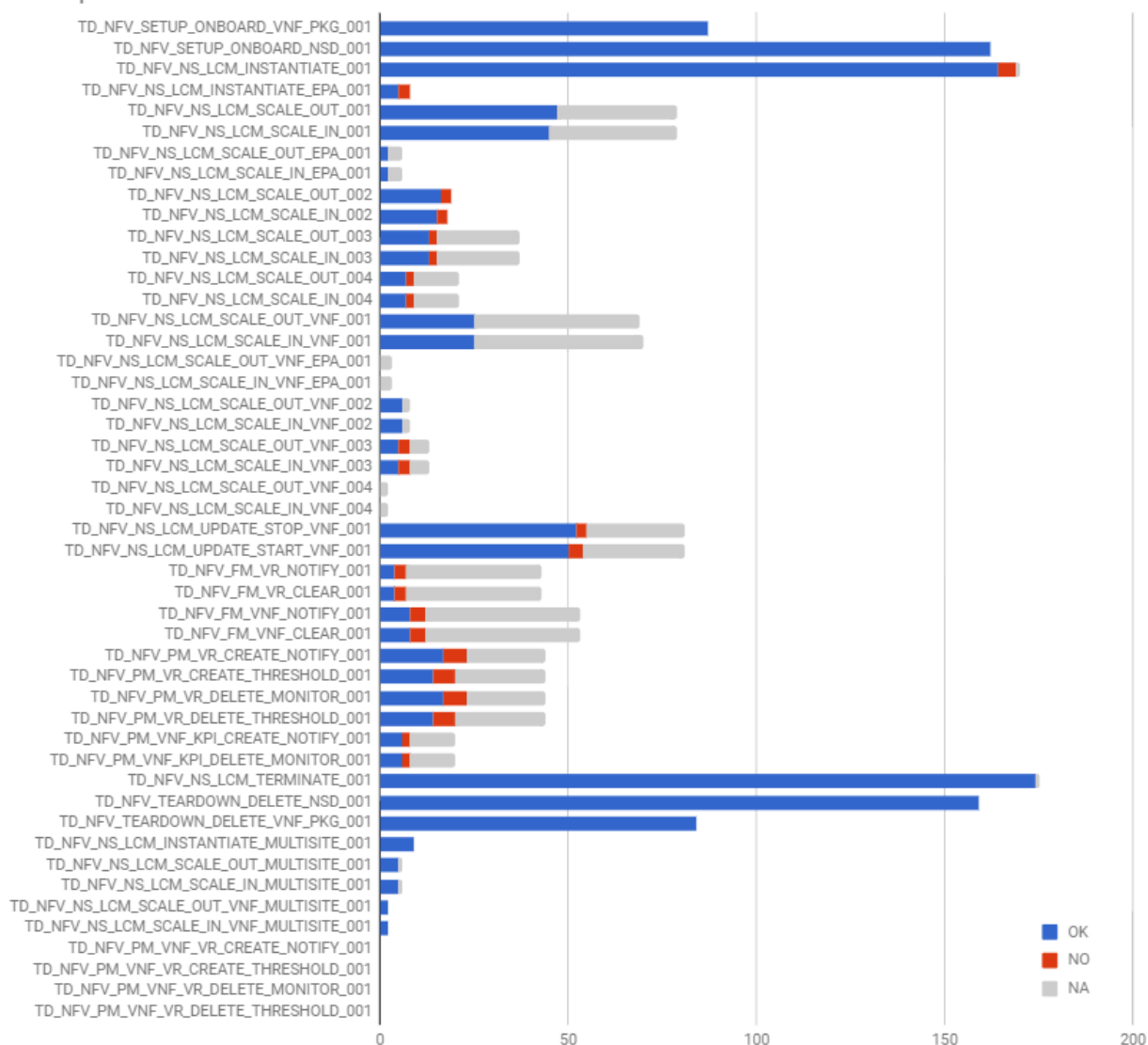
Results per Test Case
