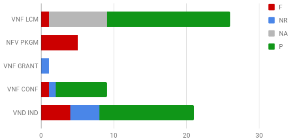
Figure 32: API Track results per interface
