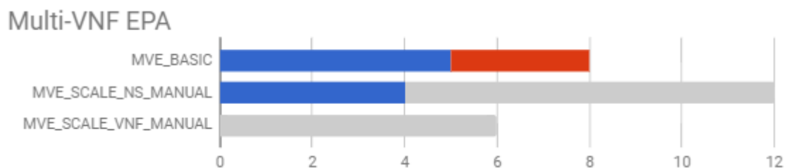
Figure 25. Results per Sub-Group (Multi-VNF-EPA)
