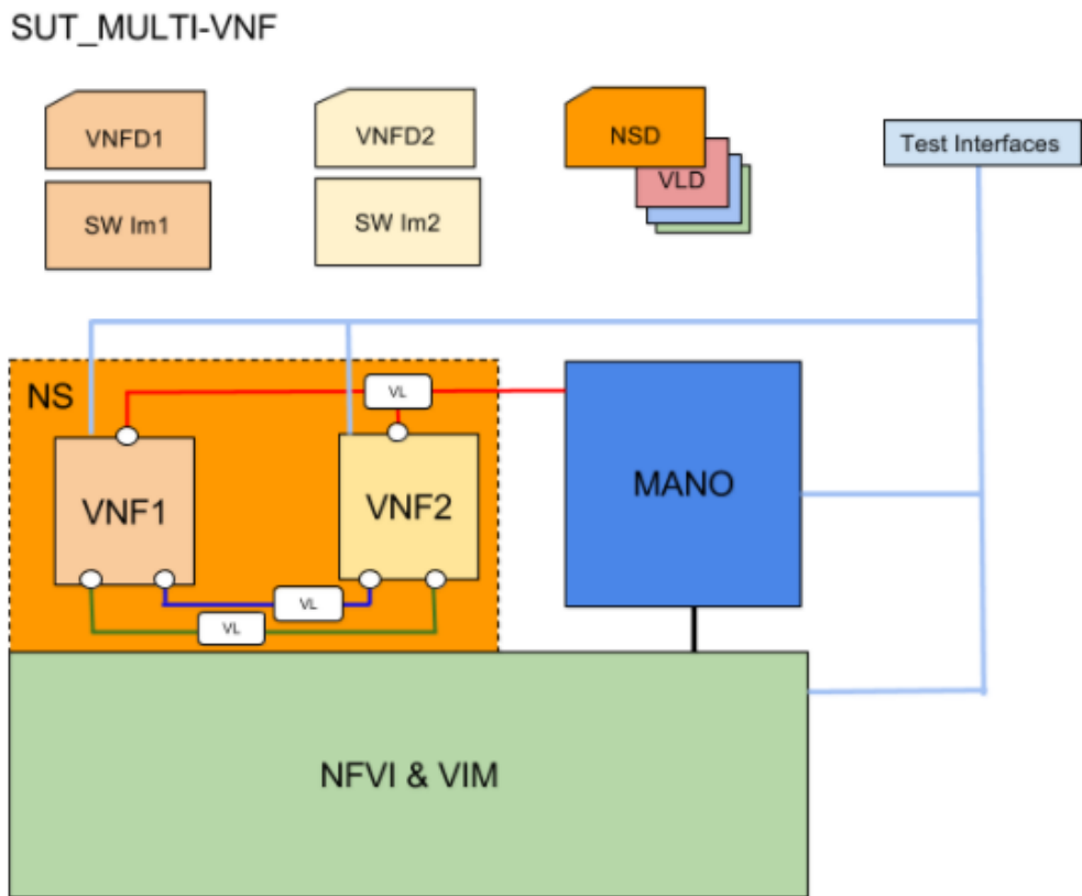
Figure 15. Multi-VNF-EPA Configuration: SUT_BASE
