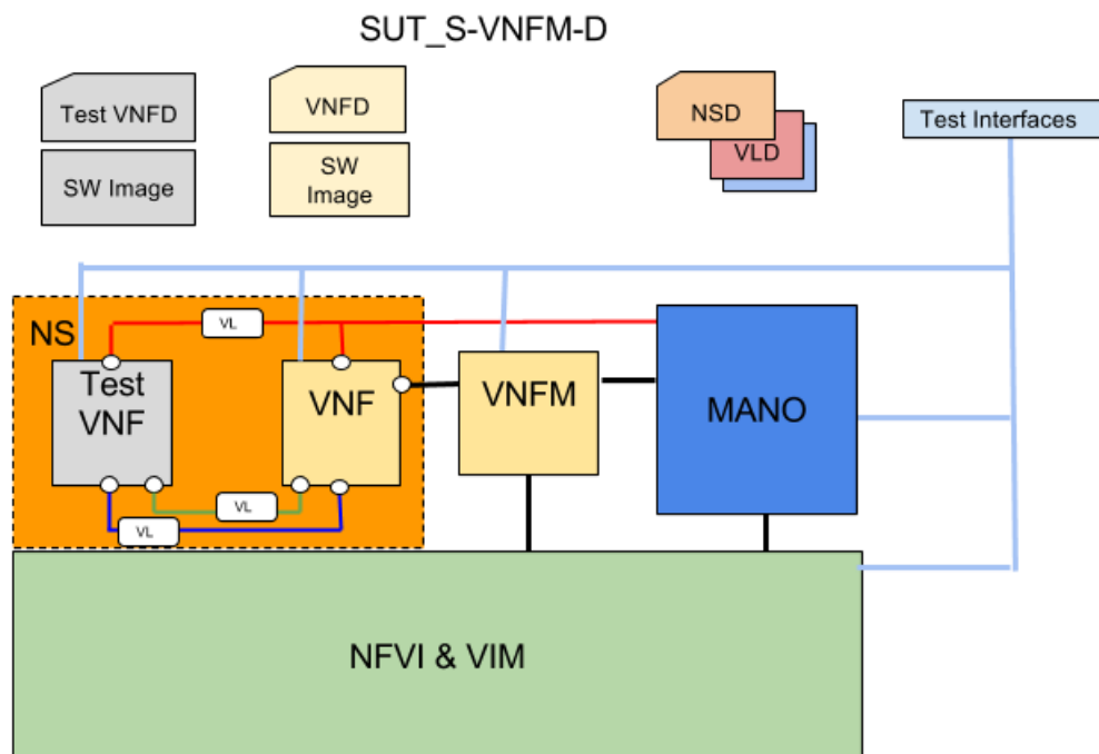
Figure 17. Specific VNFM (Direct Mode) Configuration: S-VNFM-D
