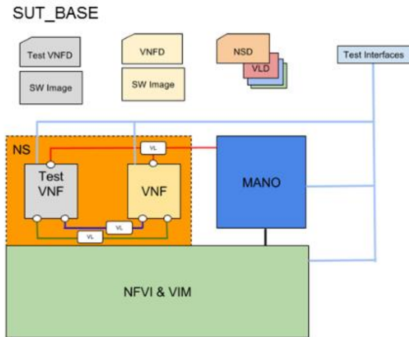
Figure 11. SUT Configuration example.
