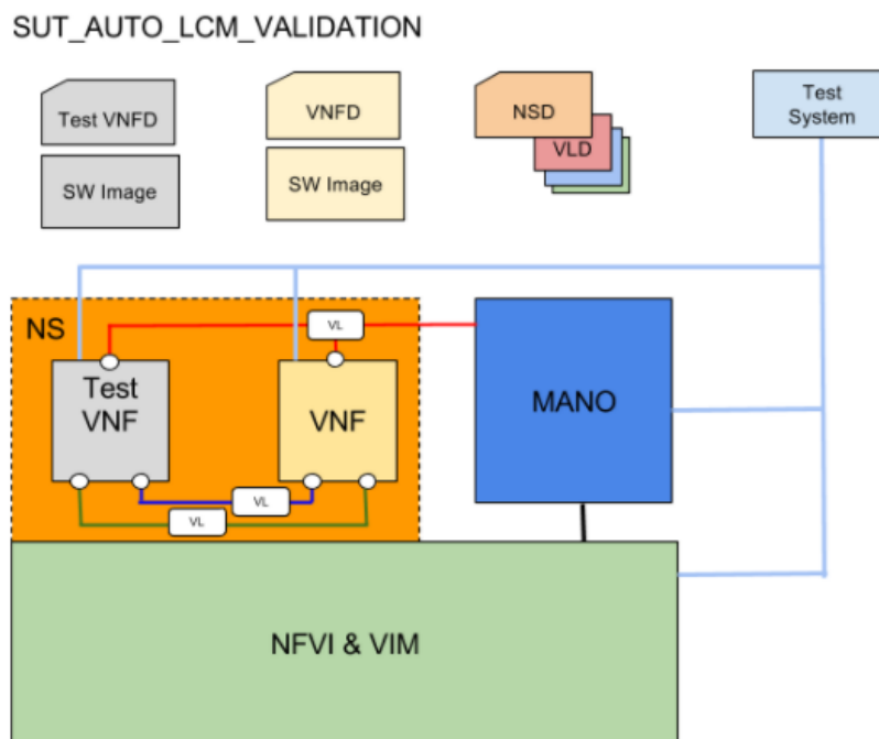
Figure 29. AUTO LCM Validation SUT Configuration: SUT_BASE
