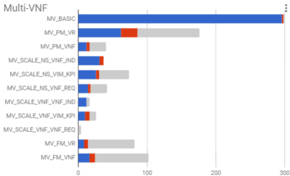
Figure 23. Results per Sub-Group (Multi-VNF)
