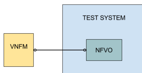
Figure 29: Test configuration SUT_1_API_VNFM_OR
