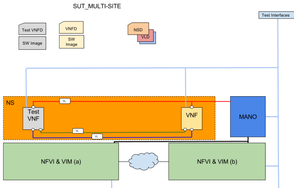
Figure 16. Multi-SITE SUT Configuration
