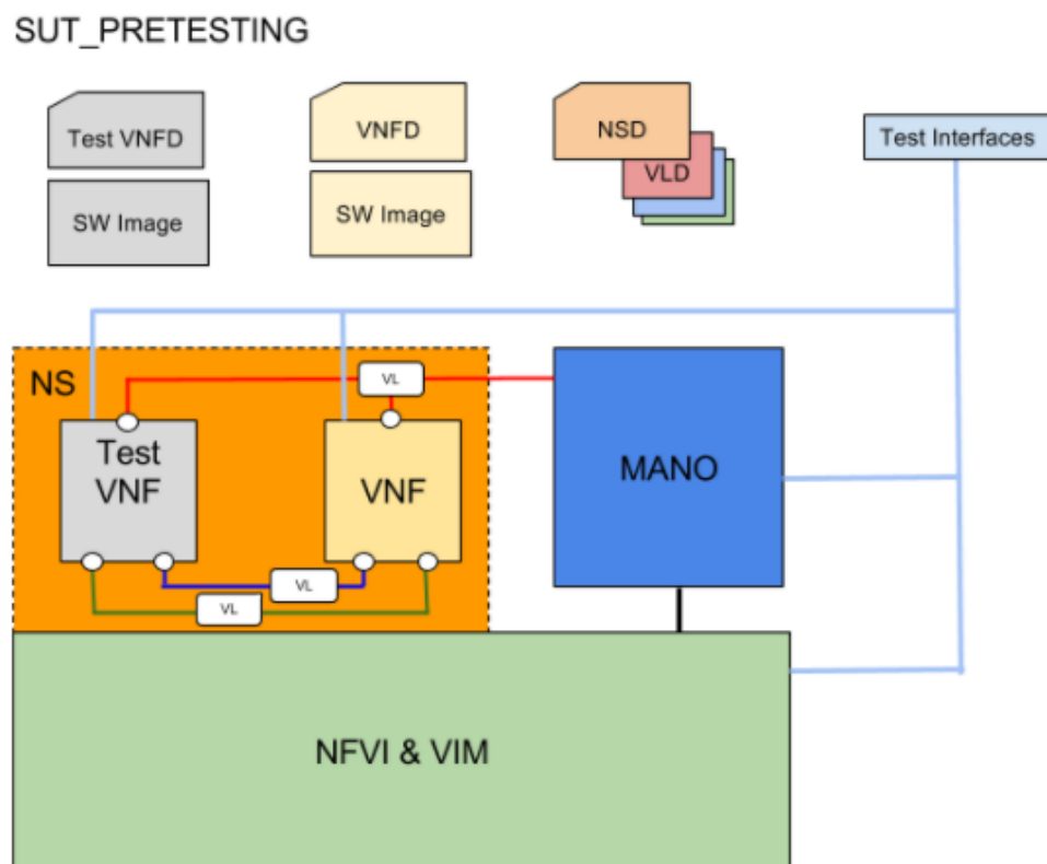
Figure 13. Pre-testing Configuration: SUT_BASE
