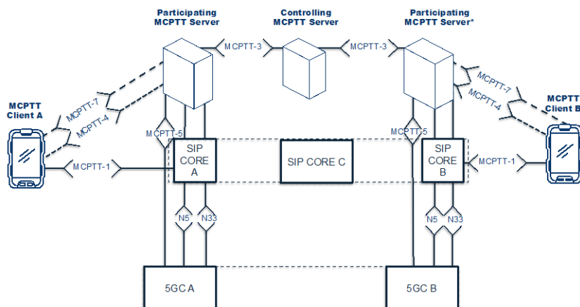
Figure 8. CFG_ONN_UNI-MC-LTE-1 configuration
