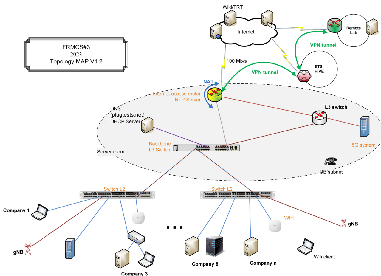
Figure 3. Remote Test Infrastructure
