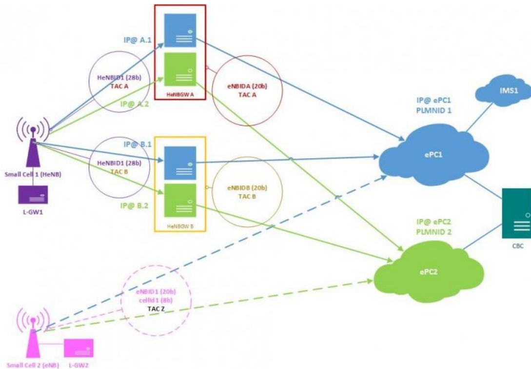
Figure 10. Network Architecture.
